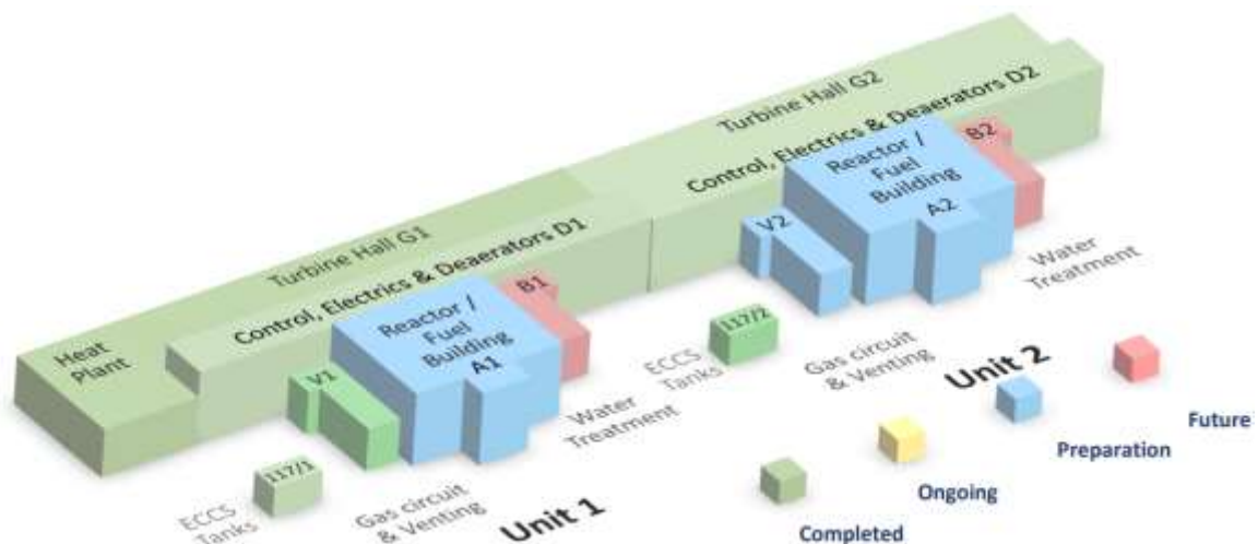
Figure 2-1 Layout of the INPP Units and the actual status of D&D works
