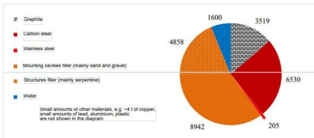
Figure 2-3 Estimated amount of R3 zone materials (tonnes, both Units)
