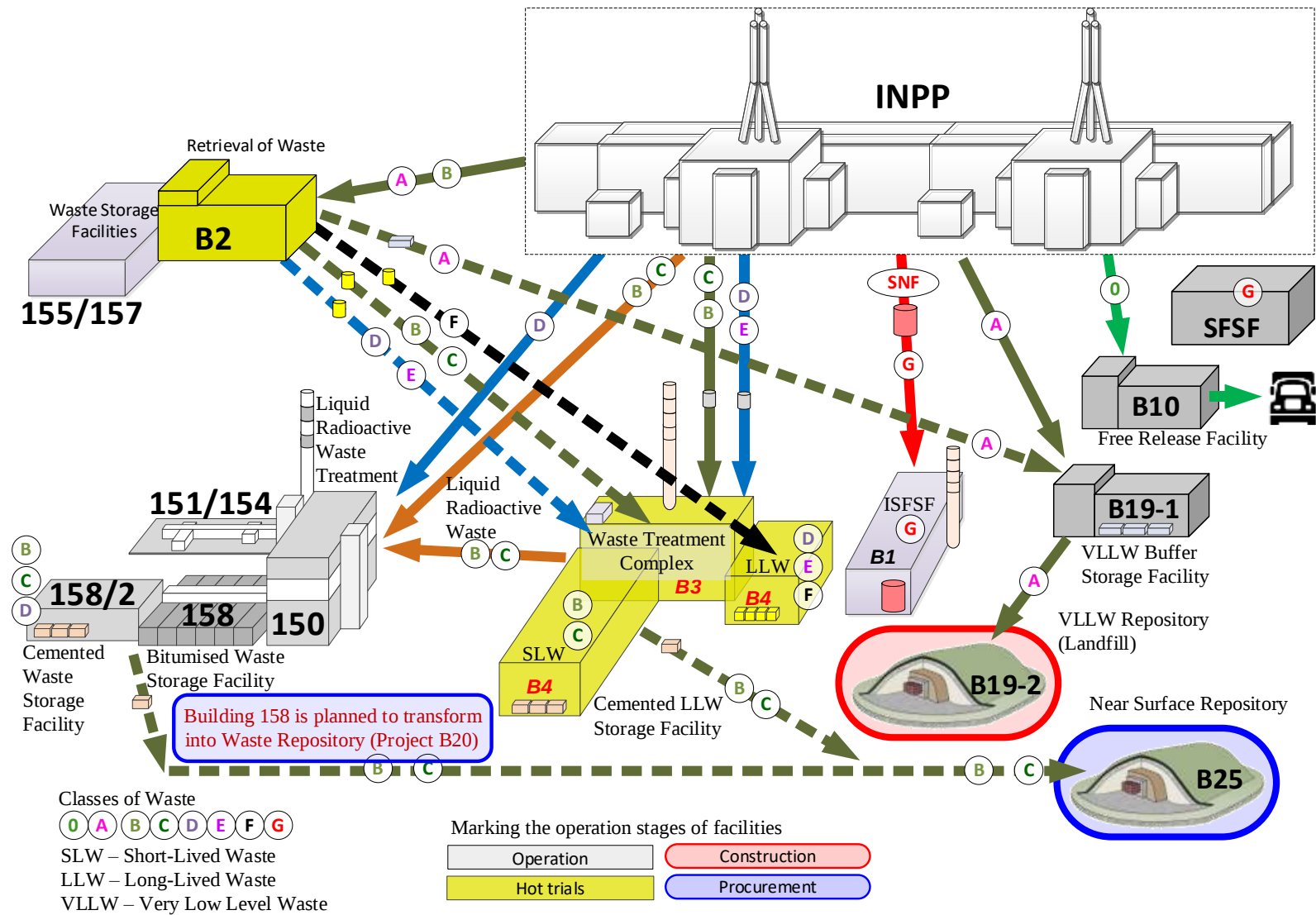
Figure 2-4 Simplified scheme of the waste management
