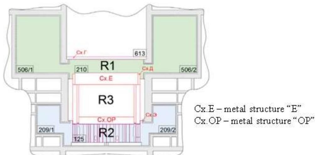
Figure 2-3 Reactor dismantling zones
