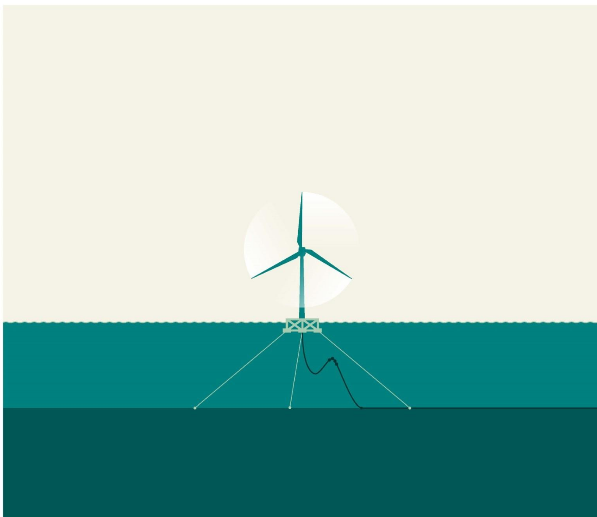
Figure 11. Floating foundation connected with a dynamic cable to accommodate the movement of the foundation. Illustrator: Tobias Green.
