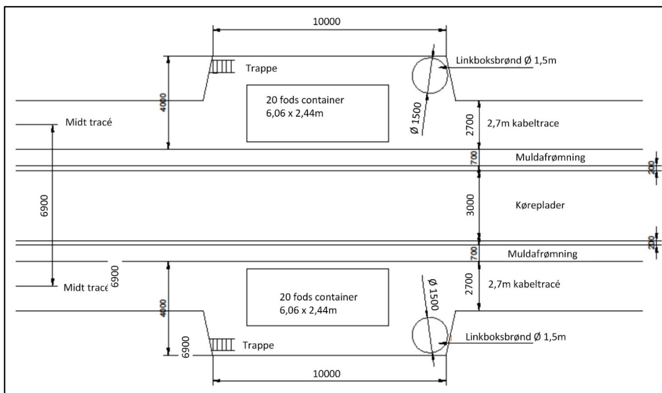
Figur 2-11 Plan af muffegrav
